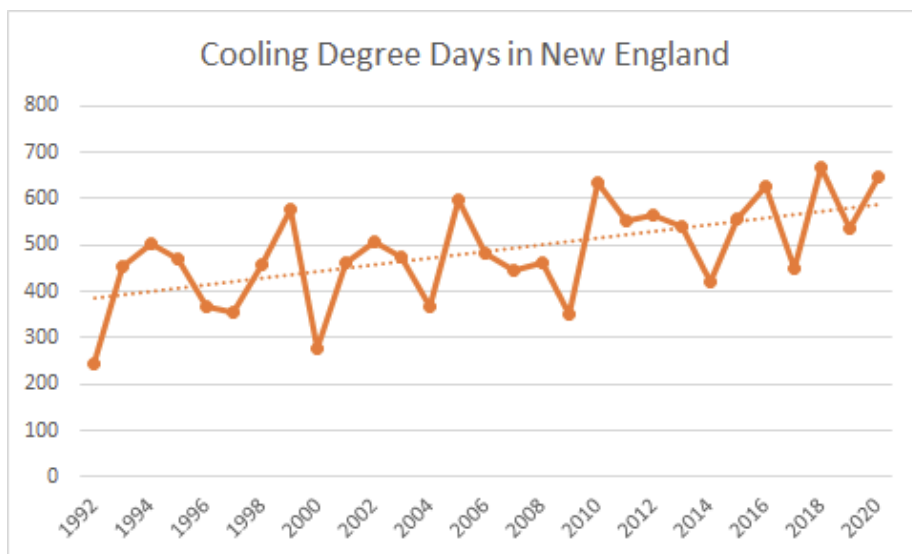
Exhibit 6-5. 5 Cooling Degree Days in New England
