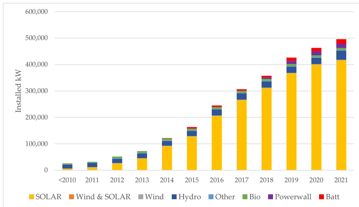
Exhibit 7-20. Cumulative installations of distributed generation resources by year, by capacity (kW)
