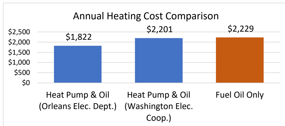
Exhibit 6-15. Heating Cost Comparison
