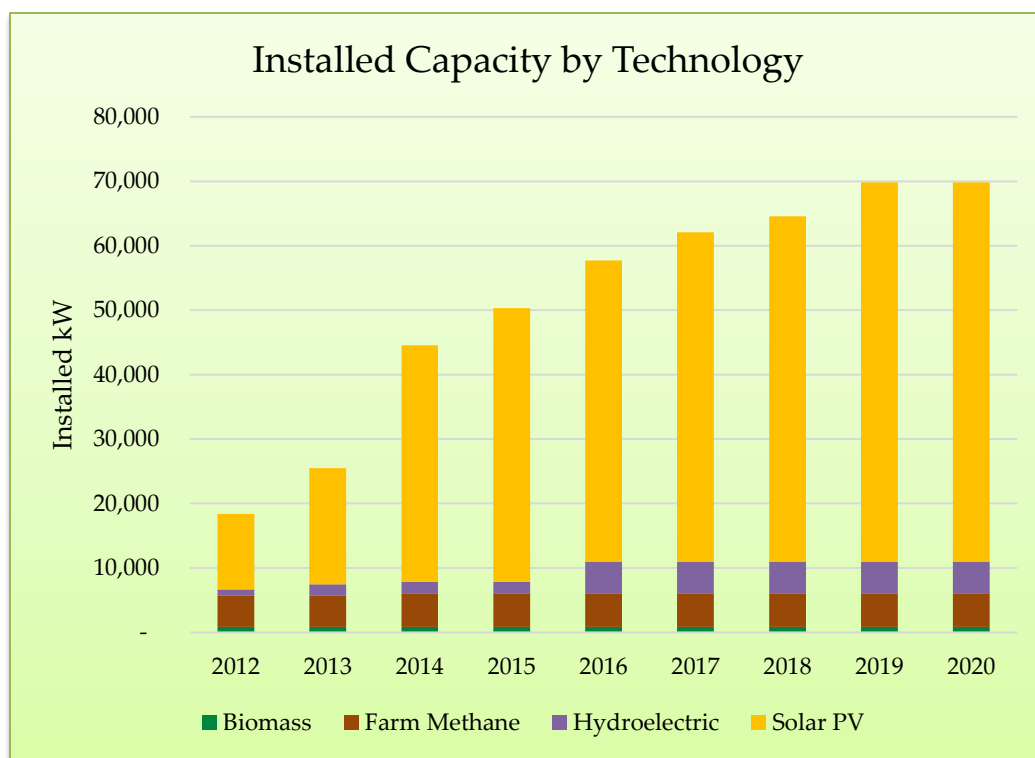
Exhibit 7-18. Installed Standard Offer Projects by Technology
