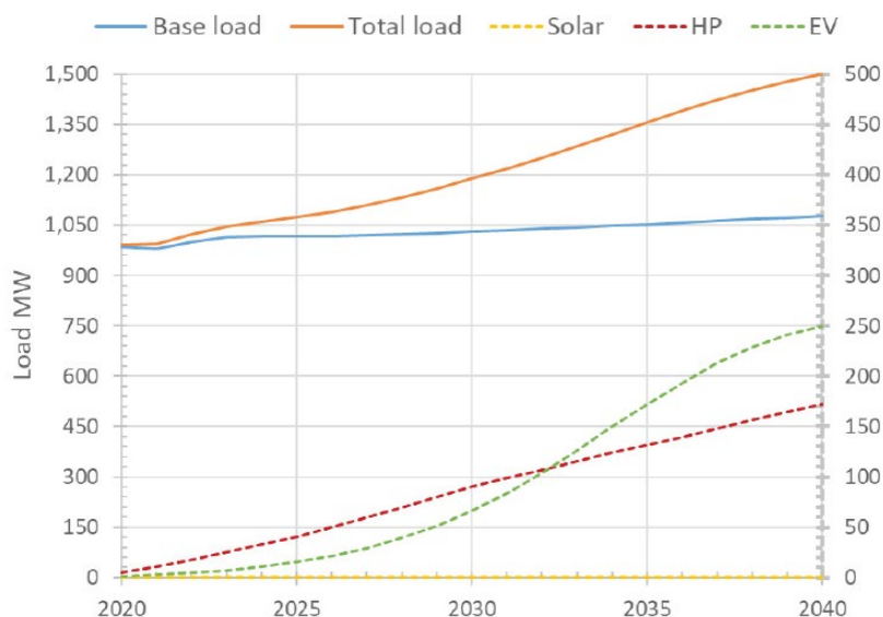
Exhibit 5-7. Projected Vermont Winter Peak Load (with Components), 2020-2040.
