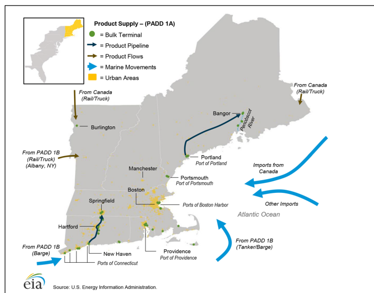
Exhibit 6-16. New England Petroleum Supply Lines
